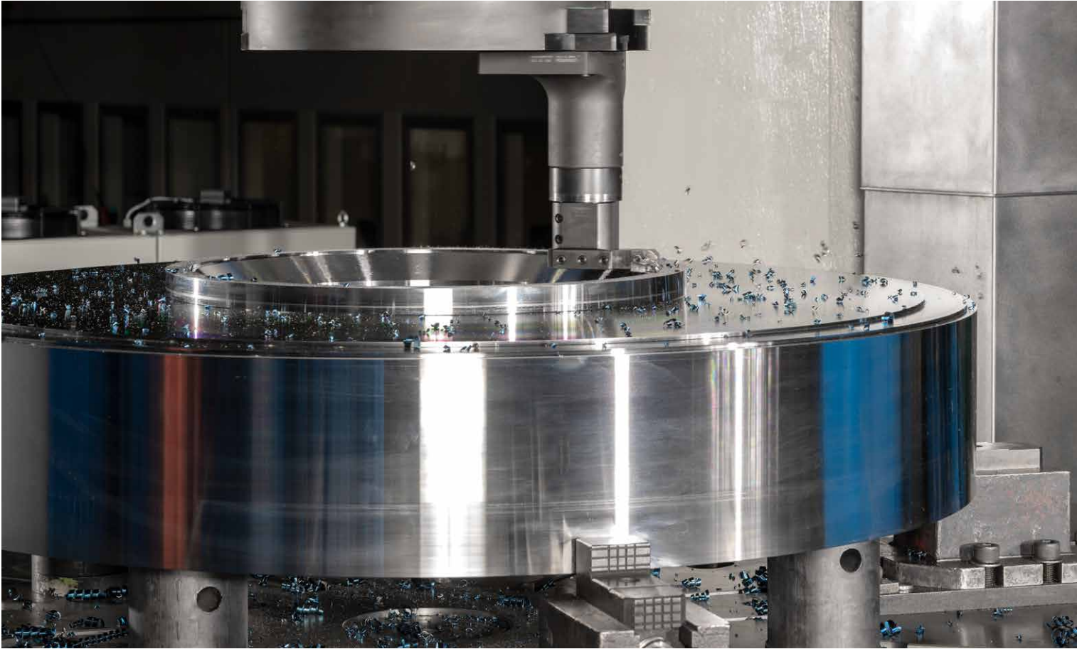
WaldrichSiegen ProfiTurn V – powerful vertical lathe for special requirements
