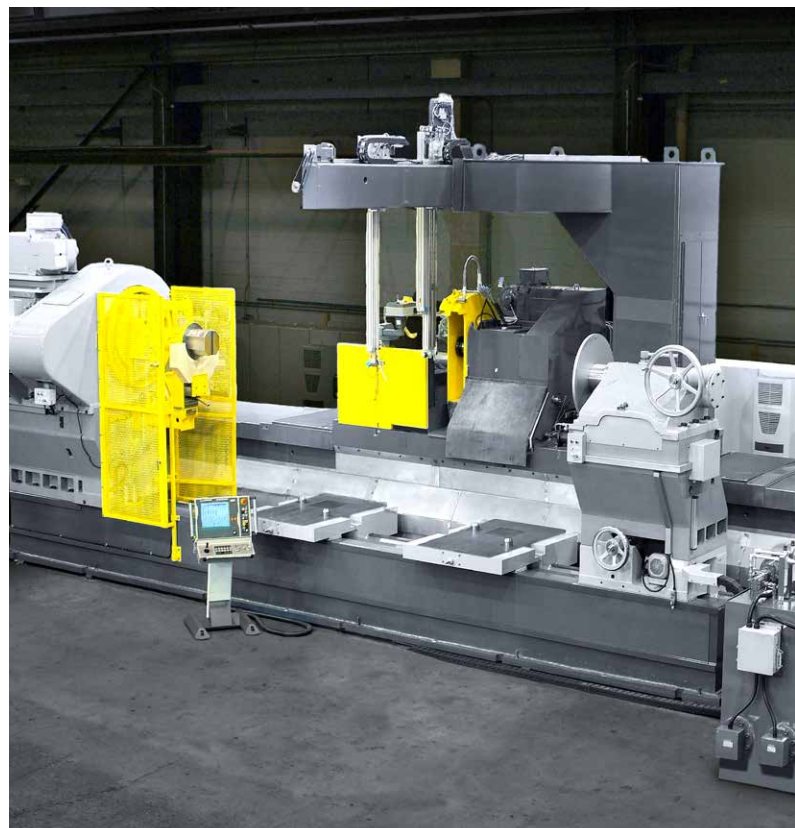
Another high quality modernization of a Mesta grinder: Performance like a new machine
